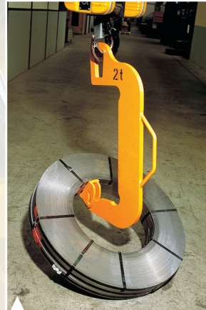
Coilkipphaken Baureihe C33 Coil Tipping Hooks Series C33
